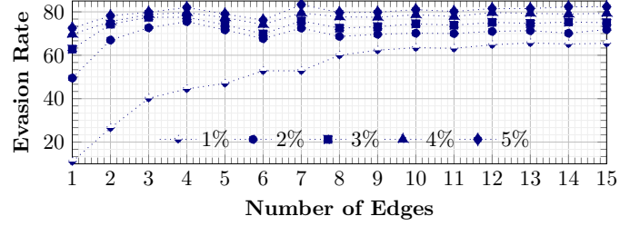
Fig. 9: SNIA evasion rate for a target model that has undergone adversarial retraining using SNIA AEs. New SNIA AEs were created to evaluate the retrained model with max perturbation caps (varying up to 5%, as shown in the legend with the different percentages) and varying edges.
