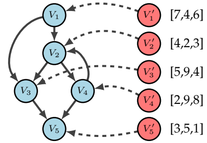
Fig. 4: SMNIA artificial node connections.
