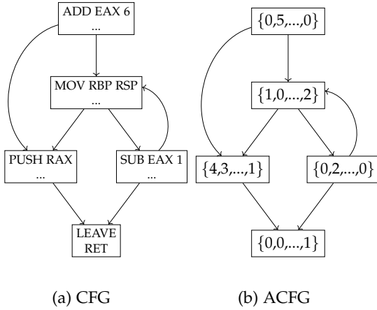
Fig. 2: CFG and ACFG developed from a software binary.
