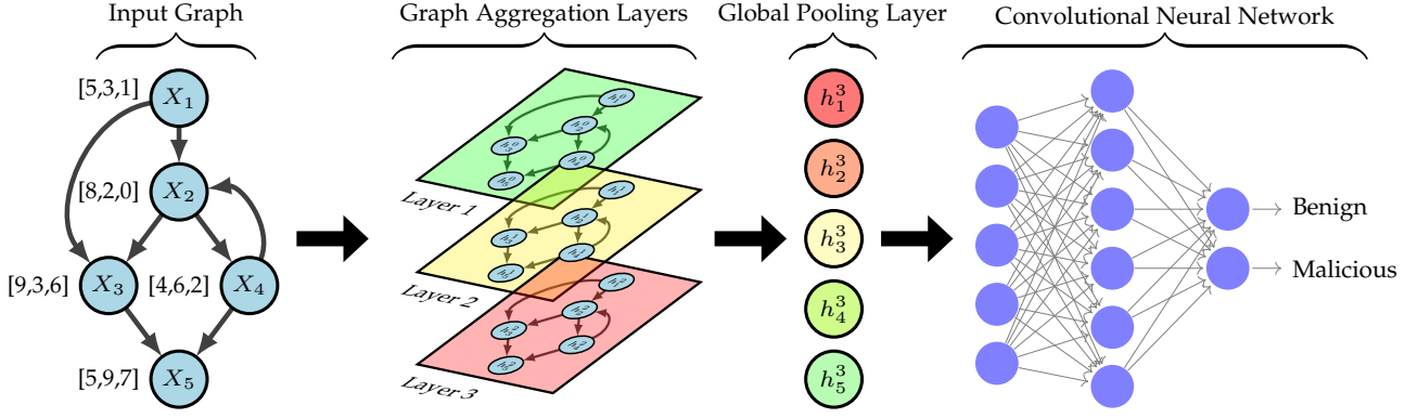
Fig. 1: An example of a typical GNN model used for malware detection (two-class classification), starting with an input graph (e.g., ACFG) that is aggregated, pooled, and convoluted to produce a final graph label.
