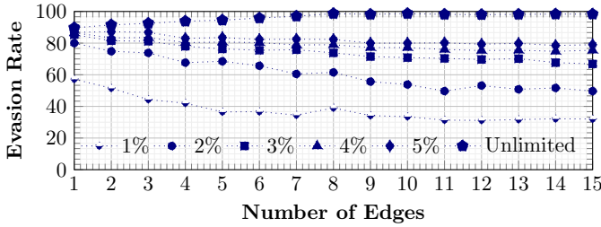
Fig. 7: SMNIA evasion rate with max perturbation caps (varying, up to unlimited, as shown in the legend with the different percentages) and a varying number of edges.
