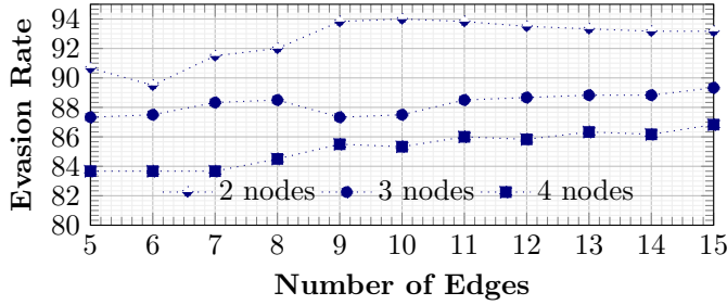
Fig. 8: SNICA evasion rate with a max perturbation cap of 5.00% under a varying number of nodes and edges.
