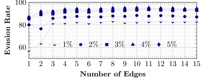
Fig. 6: SNIA evasion rate with max perturbation caps (varying, up to 5%, as shown in the legend with the different percentages) and a varying number of edges.
