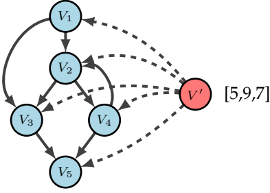
Fig. 3: SNIA artificial node connections.
