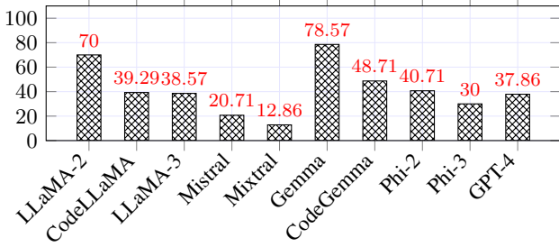
Fig. 3: Comparing AP at file-level across different models.
