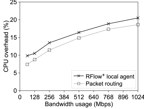
Figure 3.8: Overall CPU overhead of RFlow + local agent compares to that of packet routing only scenario by varying bandwidth utilization.
