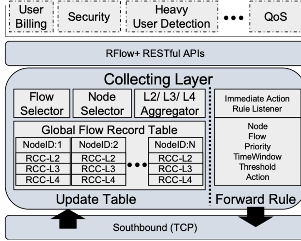
Figure 3.4: Internals of RFlow + Global Agent. The global flow record table collects and stores the flow record updates from the local agent for providing statistics accesses to northbound applications through RESTful API.
