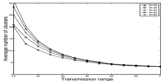
Fig. 1. Average number of clusters, max\_disp=5
