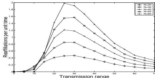
Fig. 2. Reaffiliations per unit time, max\_disp=5
