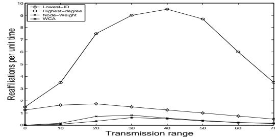
Fig. 7. Comparison of reaffiliations, N=30
