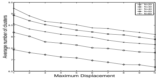
Fig. 4. Average number of clusters, tx\_range=30
