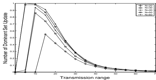
Fig. 3. Dominant set updates, max\_disp=5
