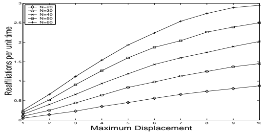
Fig. 5. Reaffiliations per unit time, tx\_range=30
