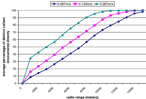
Figure 8: Average percentage of distinct neighbors encountered directly.
