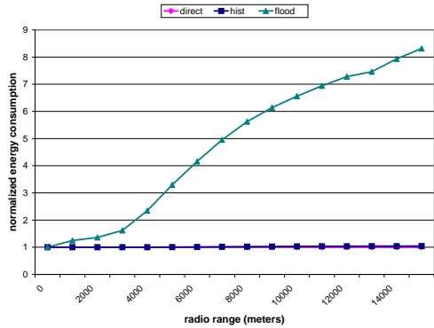
Figure 13: Normalized energy consumption for the non-resource-constrained case. The energy consumed by direct transmission is very close to that dissipated by the history-based protocol.
