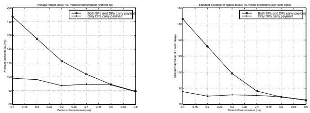
Fig. 8. Delay (left) and Jitter (right) measurements for Voice over CPN. Only DPs carry payload (curves below), and both DPs and SPs carry payload (curves above)
