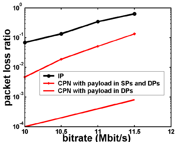
Fig. 6. Logarithmic value of the percentage of lost packets plotted as a function of link load
