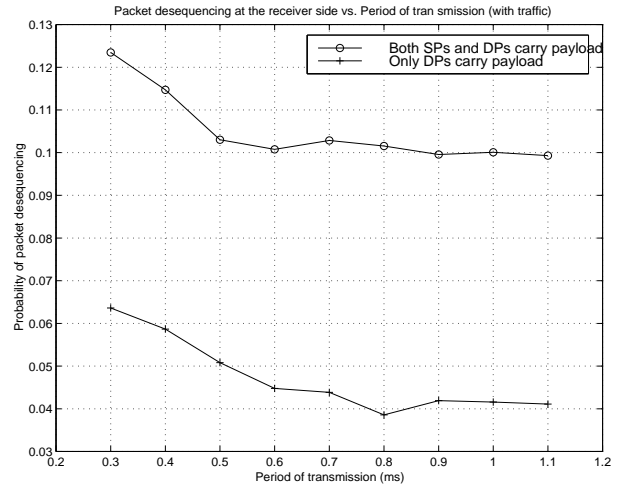
Fig. 9. Probability that a packet arrives out of sequence at the receiver: Only DPs carry payload (curve below), and both DPs and SPs carry payload (curve above)
