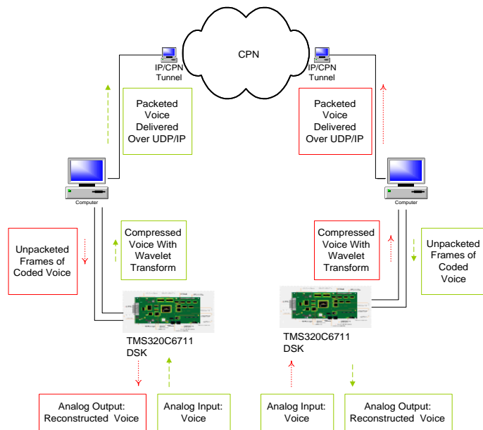
Fig. 3. Test-Bed Setup for Voice Transmission
