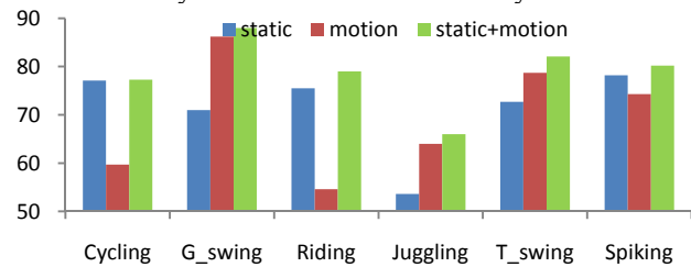
Fig. 5 Recognition performance on YouTube dataset. The average accuracy for static, motion and static+motion experimental strategy is 71.4%, 69.6% and 78.1% respectively.
