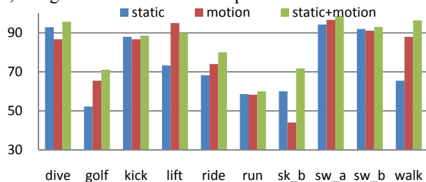
Fig. 4 Recognition performance on UCF sports dataset. The average accuracy for static, motion and static+motion experimental strategy is 74.5%, 79.6% and 84.5% respectively.
