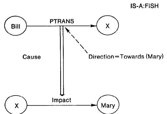
Figure 5-2 A conceptual dependency diagram from Pat Hayes (1977)
