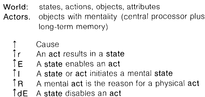
Figure 5-3 Conceptual Dependency model (after Schank & Abelson, 1977)
