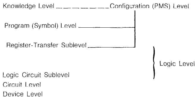
Figure 3-3. New version of computer system levels
