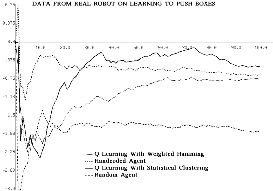
Figure 28: Real data on learning to push boxes
