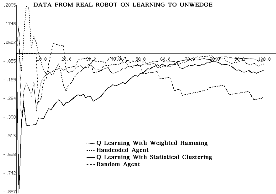
Figure 30: Real data on learning to unwedge
