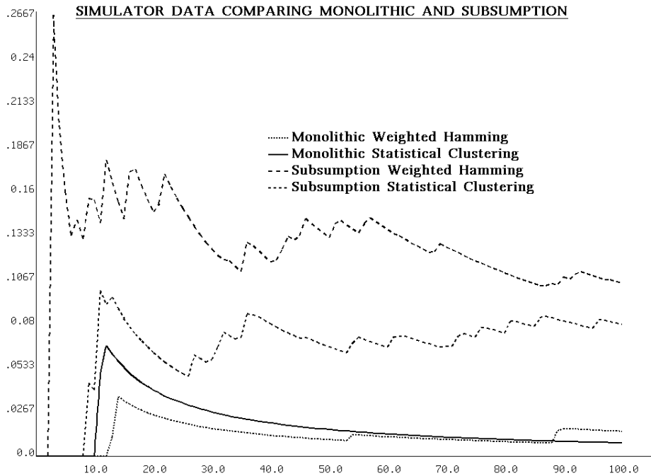
Figure 34: Simulator data comparing the monolithic and subsumption learners
