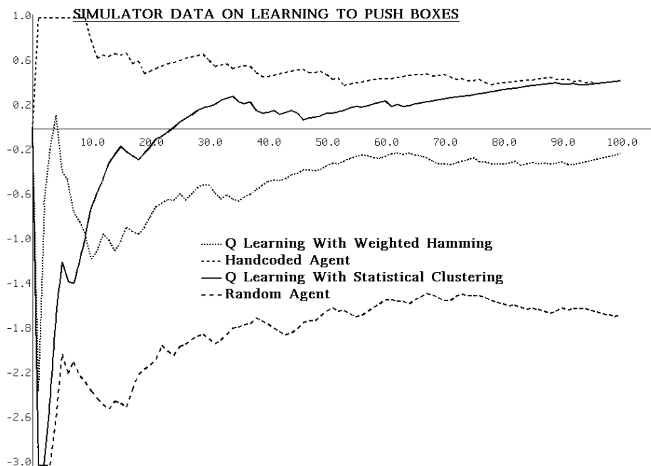
Figure 27: Simulator data on learning to push boxes
