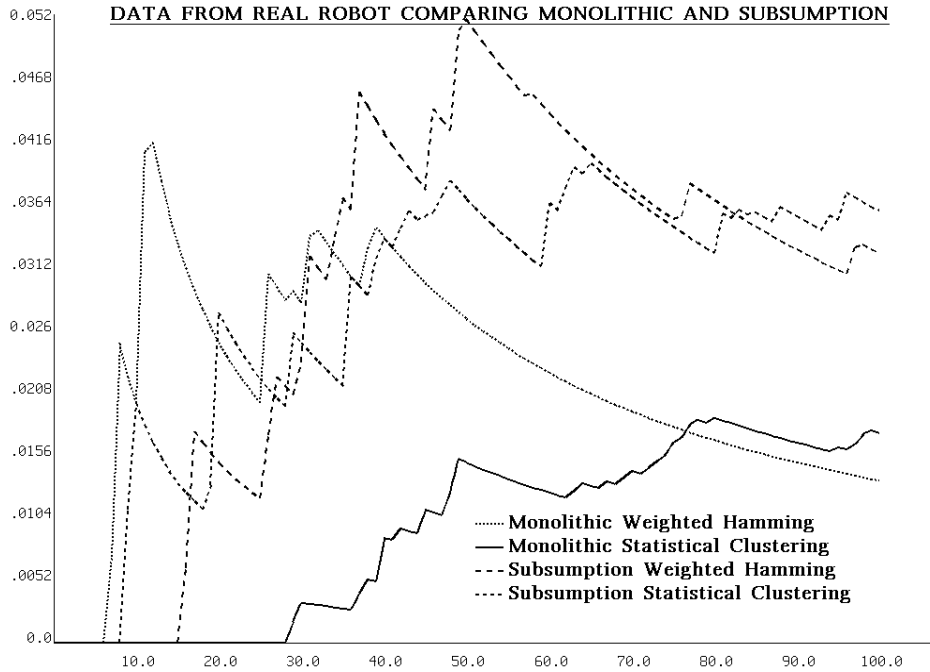
Figure 35: Data from real robot comparing the monolithic and subsumption learners
