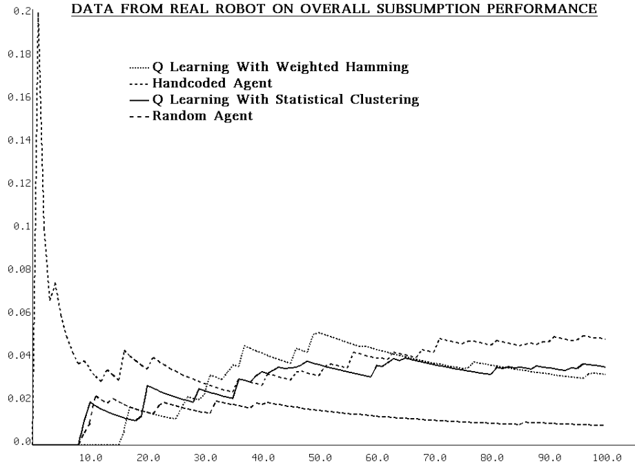
Figure 33: Real data evaluating the subsumption approach using the monolithic reward function
