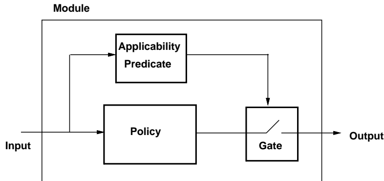
Figure 6: A Module in a Subsumption Architecture
