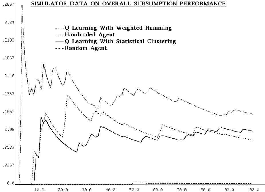
Figure 32: Simulator data evaluating the subsumption approach using the monolithic reward function
