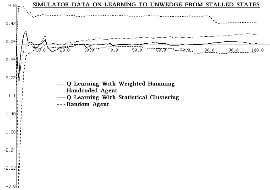
Figure 29: Simulator data on learning to unwedge
