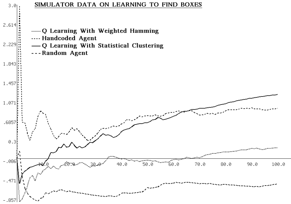
Figure 25: Simulator data on learning to find boxes
