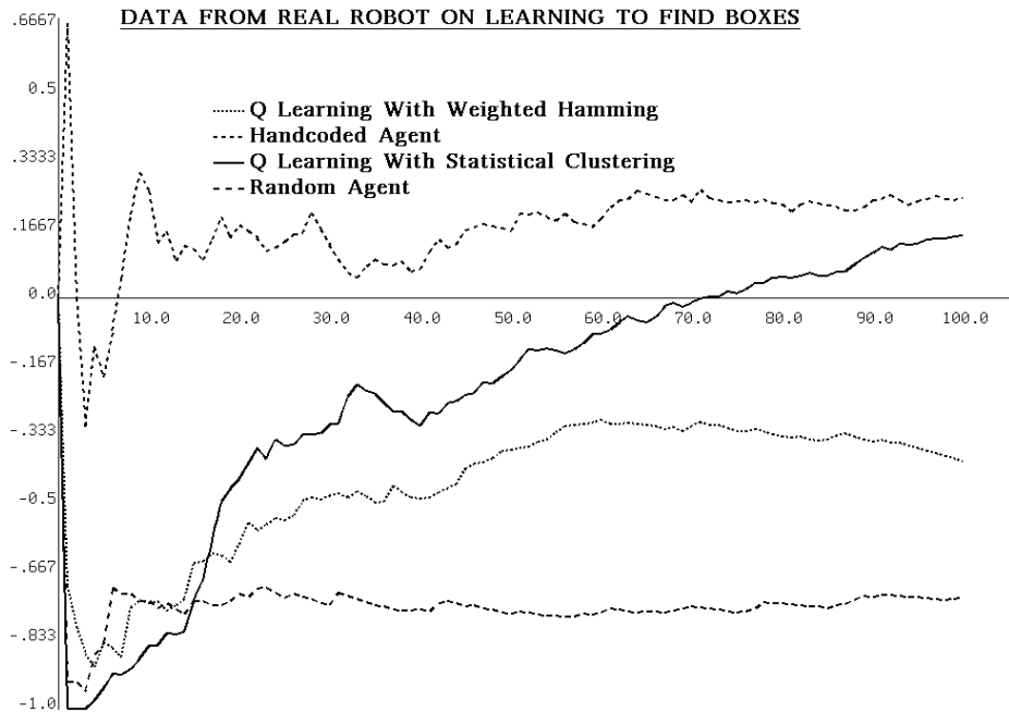
Figure 26: Real data on learning to find boxes
