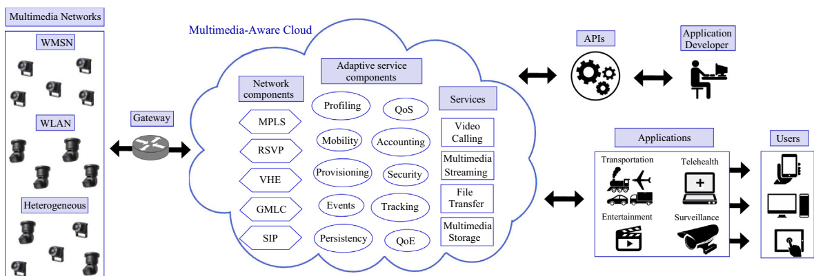
Fig. 6. Multimedia-aware cloud's middleware architecture.
