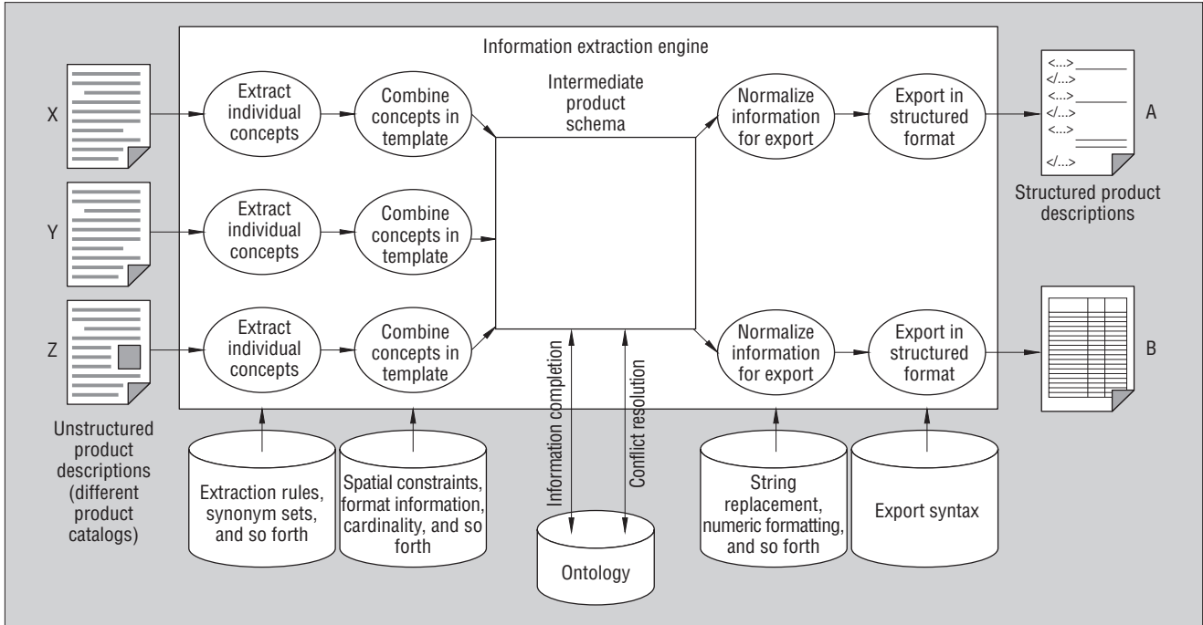
Figure 4. A sketch of the information extraction engine.
