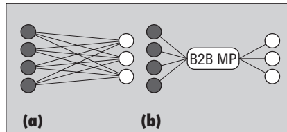
Figure 1. Preventing exponential growth in the number of mappings: (a) direct communications between m suppliers and n customers = n * m mappings; (b) mediated communications between m suppliers and n customers = n + m mappings.
