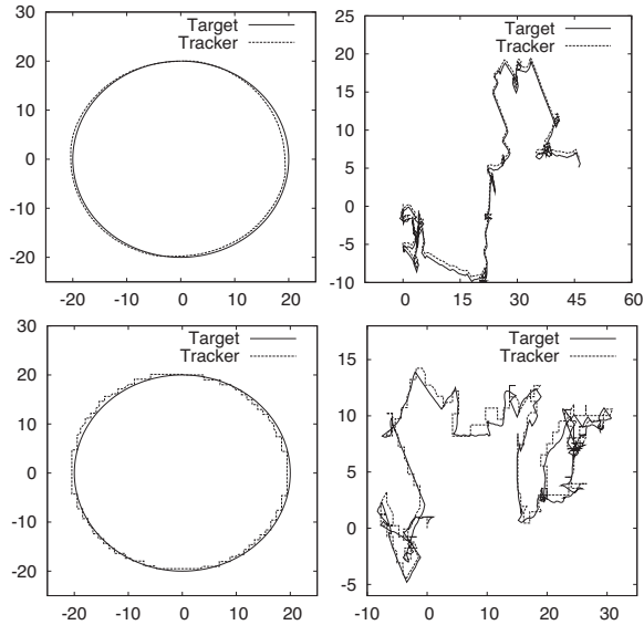
Figure 1: Performance with (top row, M-VAR) and without (bottom row, M-NOVAR) inter-agent variation.
