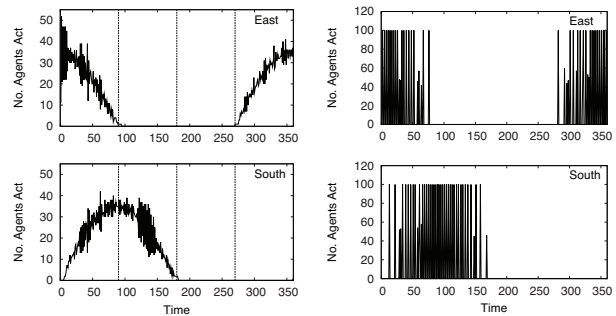
Figure 2: Number of agents that act in each timestep for the circle tracking problem using M-VAR (left column) and M-NOVAR (right column).
