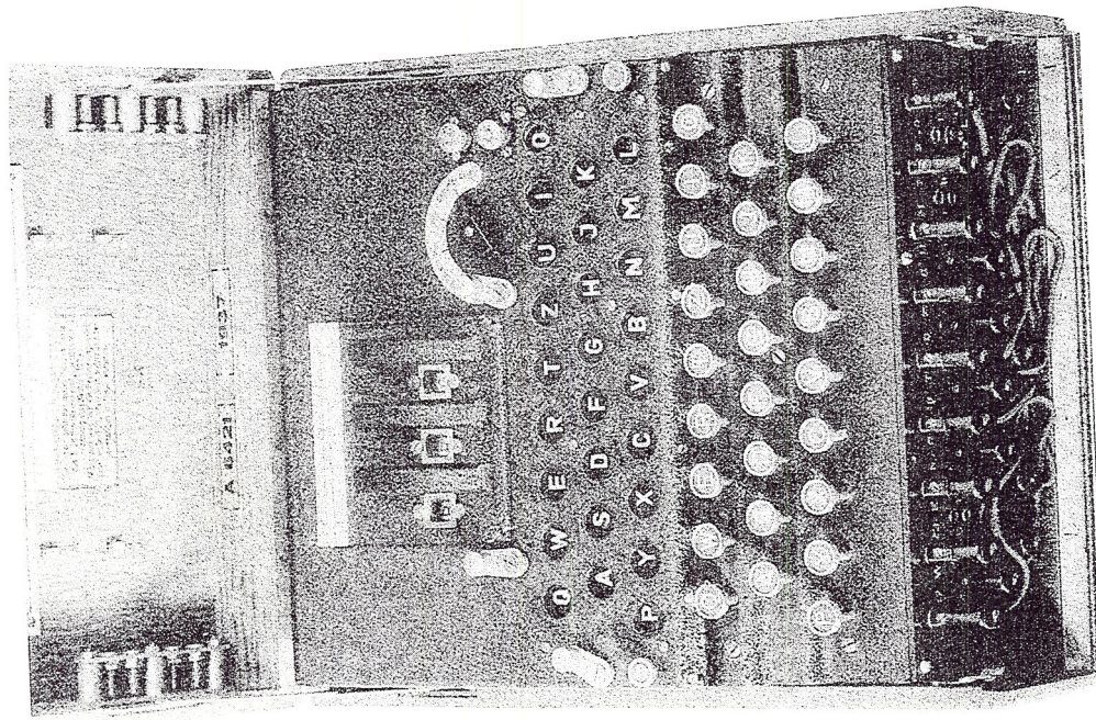
Figure 39 An army Enigma machine ready for use.
