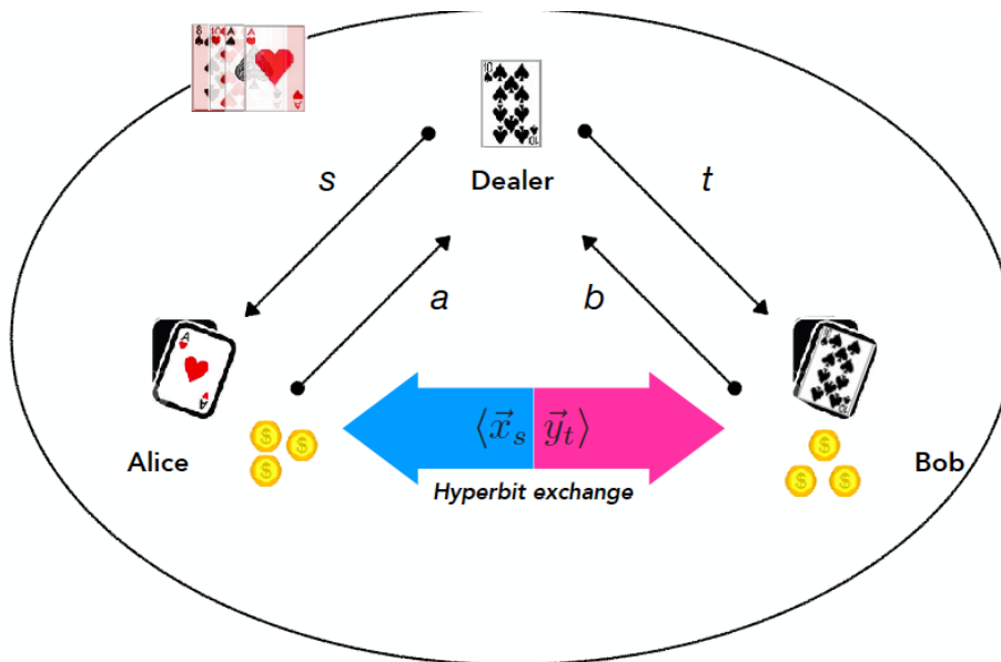
FIG. 1. An illustration of the information exchange and game play considered for this paper. The dealer sends private information (face down cards) s and t to Alice and Bob, respectively, while Alice and Bob respond with single bit actions (hit or stand) a and b . Bob uses public classical information (face up cards and action a from Alice) to optimize his choice of action b . Communication can also be conveyed through measurements by Alice and Bob on shared quantum entanglement. The contents of a finite-sized shoe (4 cards in the figure) is known to the table, although the order of the cards is not.
