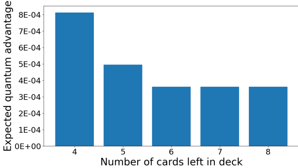
FIG. 4. The expected advantage amount plotted as a function of the shoe size. Note that the expected advantage seems to fall off and then plateau for larger deck sizes.
