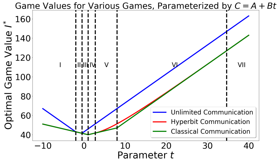
FIG. 2. A sweep of the game value for the various strategies considered, with the game parameterized by C = A + Bt . Note that seven regions are labeled for categorically different regimes; see the main text for details.
