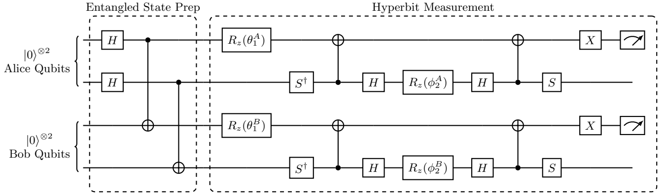
FIG. 3. Quantum circuit for the optimal hyperbit strategy when Bob and the dealer have face up cards 9 and 10, respectively, and the shoe contains cards [A, A, 8, 10]. The \theta and \phi rotation angles for both Alice and Bob are specified in Table I and depend on which facedown card each player is dealt. It is important to note that Alice and Bob’s measurements, which are conventionally 0/1, must be converted to -1/+1, and that Bob’s action is based on the product of the two measurements.
