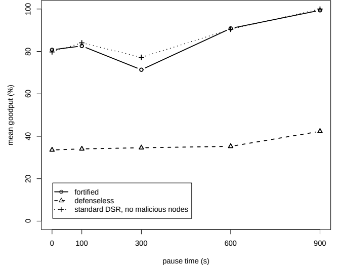
Figure 6: Goodput expressed as the ratio of received to sent packets, 50 nodes, one third malicious, 20 simulation runs.
