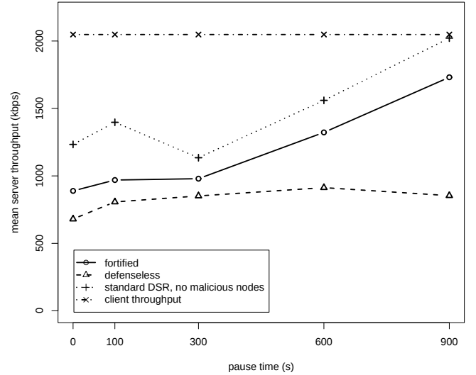
Figure 8: Client and server throughput in a network of 50 nodes with one third malicious, 20 simulation runs.
