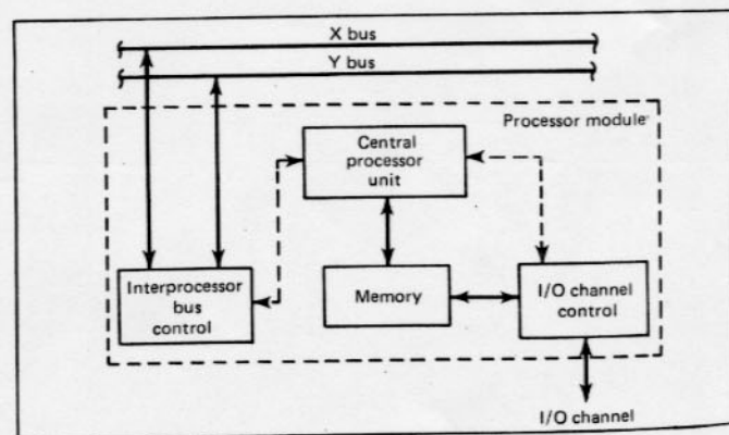
Fig. 5. Tandem 16 processor organization.
