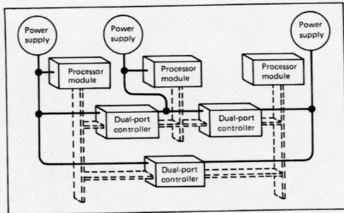
Fig. 3. Power distribution.
