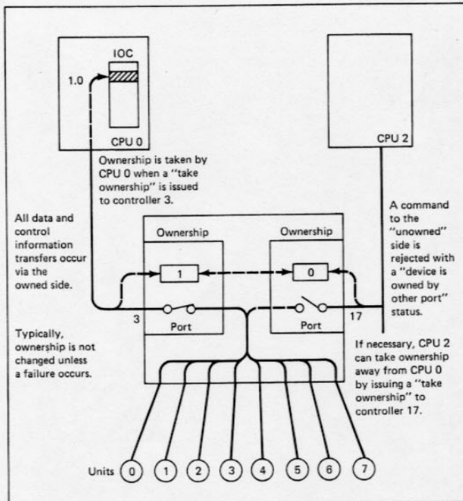
Fig. 11. Ownership circuitry.
