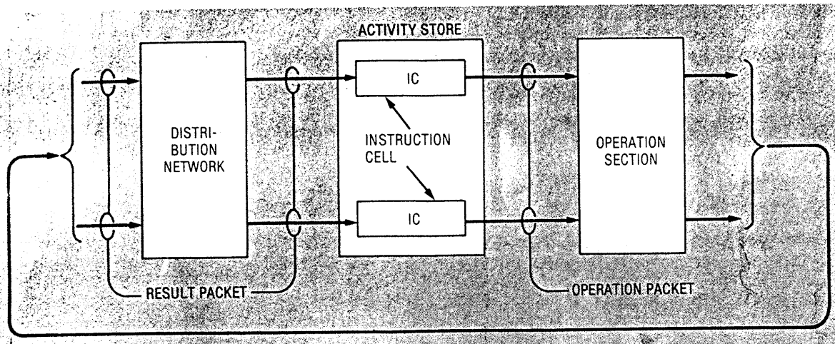
Figure 13. Genesis of the cell block architecture.
