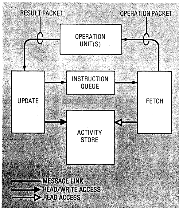
Figure 10. Basic instruction execution mechanism.
