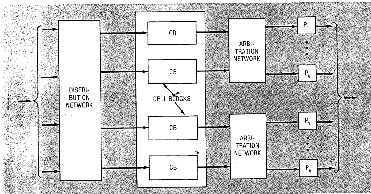
Figure 14. Practical form of the cell block architecture.
