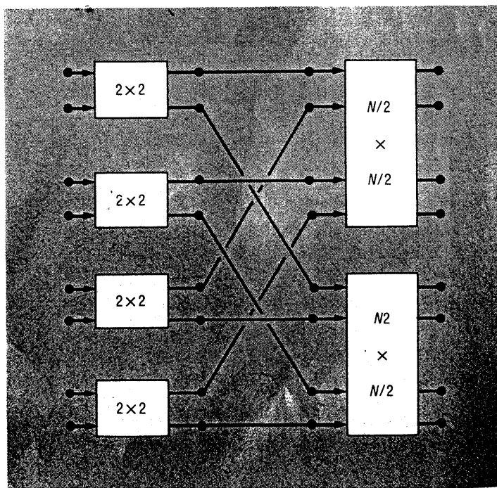
Figure 12. Routing network structure.
