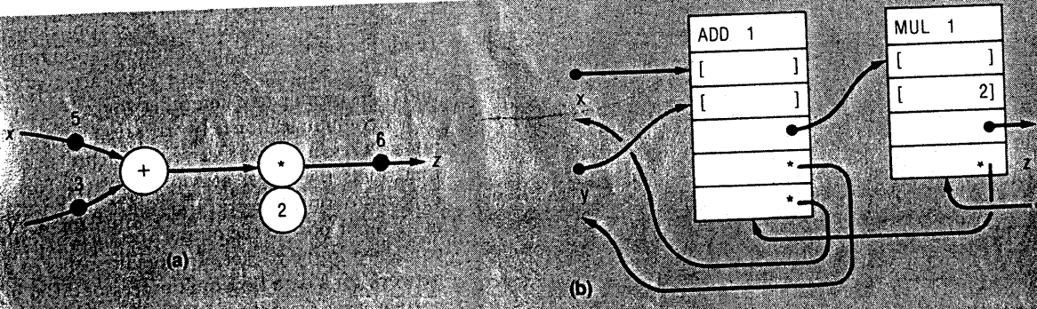
Figure 9. Pipelining in a data flow program (a) and its implementation (b).
