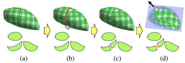
Figure 6: Insertion of a seam line. (a) Before drawing a line. (b) After drawing a line. (c) The seam line's two endpoints snap at other seam lines. (d) After pulling the seam line.
