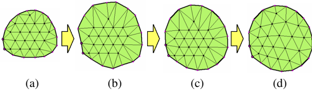
Figure 13: Updating the 2D mesh geometry. (a) before deformation. (b) boundary vertices are moved. (c) smoothing is applied to the boundary. (d) Laplacian smoothing is applied to the internal vertices.
