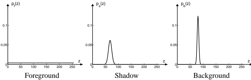
Fig. 3. L learnt emission models. Shown is a set of emission models for one pixel location. The distributions p_f , p_s and p_b model the intensity distributions for all three states foreground, shadow and background. It should be noted that the emission models can vary between pixel locations.
