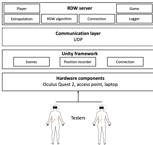
(b) Software/hardware architecture representation
