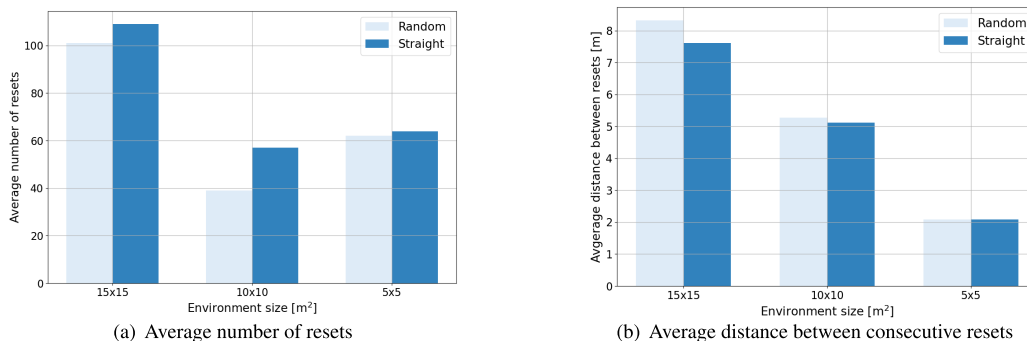
FIGURE 7. RDW performance for a single-user system in different VEs and for different sizes of the tracking space without introducing the proposed generic design enhancements.
