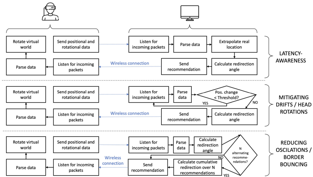
FIGURE 3. High-level designs of the RDW improvements.
