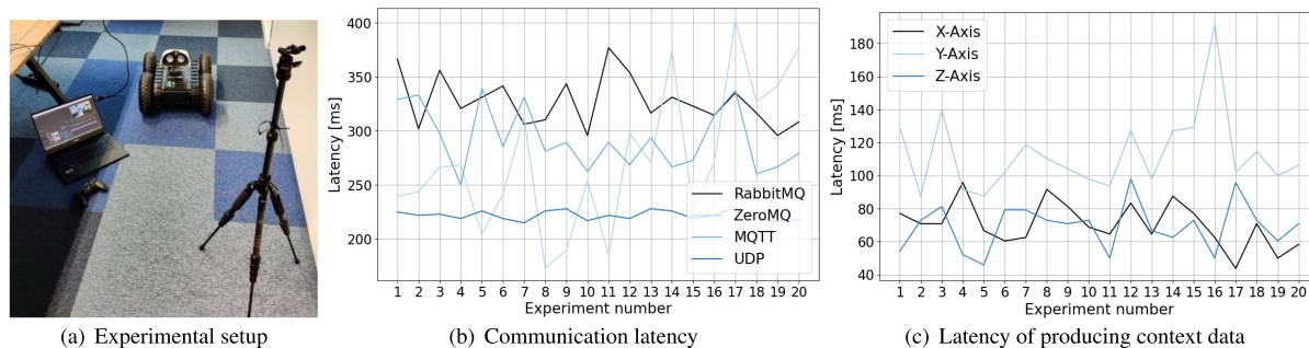
FIGURE 4. Capturing the end-to-end latency for instantiating latency-aware RDW.
