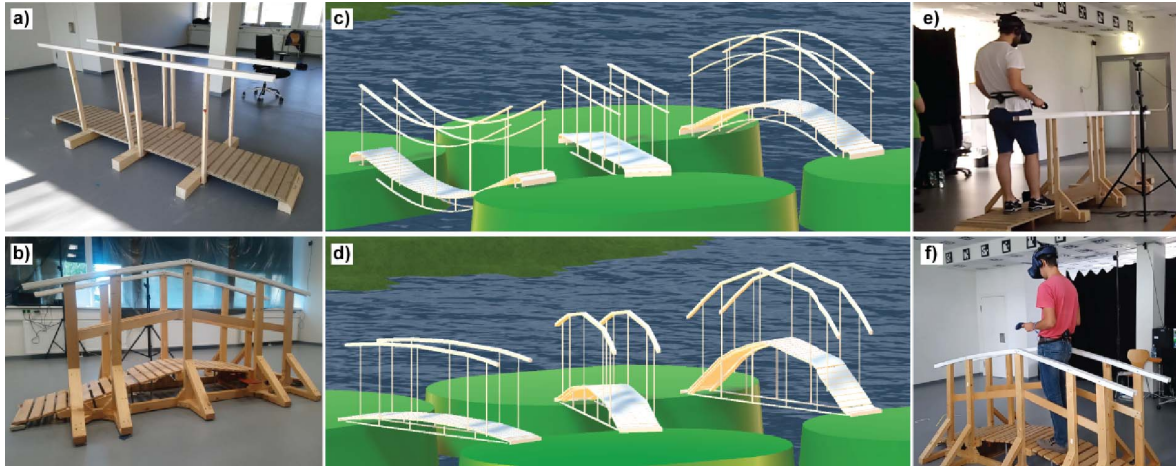
Figure 1: Simulation of smooth uneven surfaces in VR with different physical props: Study 1 (top) - we used a flat physical bridge (a) and simulated hanging (concave) and convex bridges (c). Study 2 (bottom) - we used a convex physical bridge (b) and simulated different convex virtual bridges (d) - lower and higher than the physical bridge. Images (e) and (f) show participants using our VR setups during the studies.
