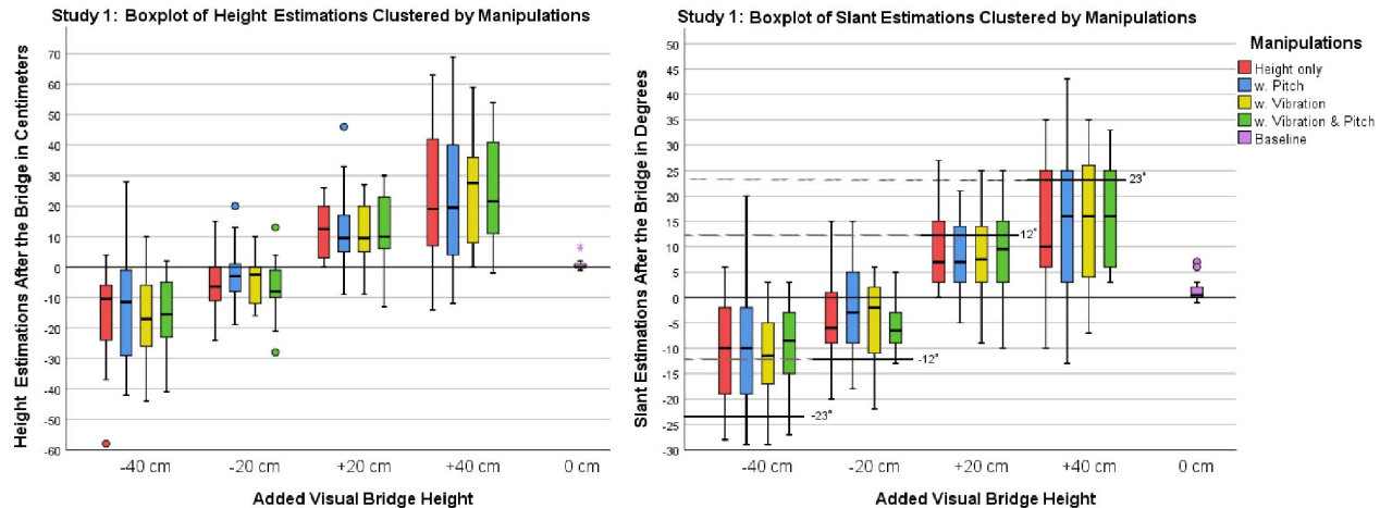
Figure 4: Study 1: Clustered boxplots for the heights (left) and slant (right) estimations for the flat physical bridge. Added visual height denotes the maximum additional height added to the virtual bridge model that replicated the real bridge. The estimations are done relative to the start of the bridge (12 cm off the ground). Slant graph includes the indication of the maximum slant of virtual bridges in accordance with the value of added visual height.
