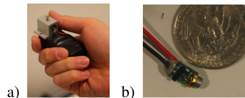
Figure 11. a) Our handheld Speckle Projector consists of a 50 mW laser (780 nm), diffuser (80°) and battery. With our speckle sensors it has a 3 m range. b) The laser diode is only a few millimeters wide and could be integrated into various hardware configurations.
