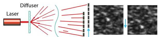
Figure 4: The speckle pattern motion can be tracked with image processing algorithms as the speckle sensor or projector move.
