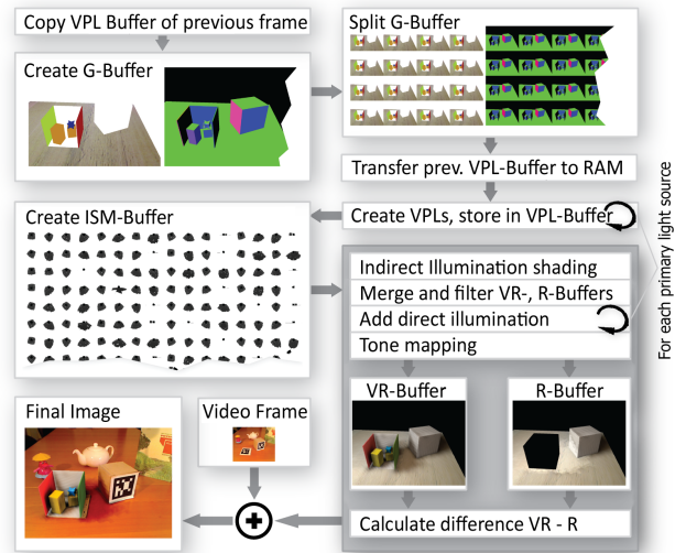
Figure 3: This figure shows the algorithm outline. A G-Buffer is created and afterwards split to reduce shading costs. The primary light sources generate VPLs from which ISMs are created. The VR- and R-Buffers are created in parallel, while the shading computation is performed only once. After some finishing steps like merging, adding direct illumination and tone mapping, the video frame is added to the difference between the VR- and R-Buffers.
