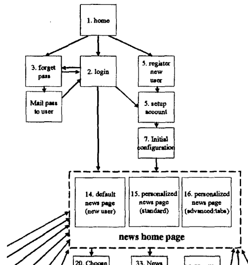
Figure 2. Part of a site map for a news web site. Site maps show entire web sites at a low level of detail.
