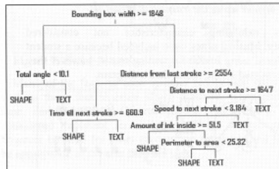
Figure 3: Classification tree for text and shape divider.
